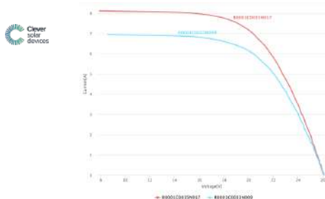
Detailed modules IV curves & comparisons
