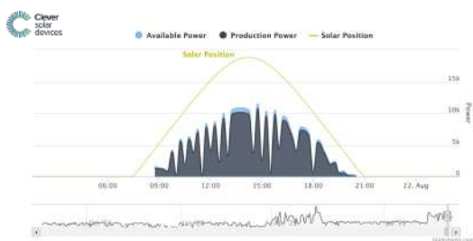
Available power vs. Production power
